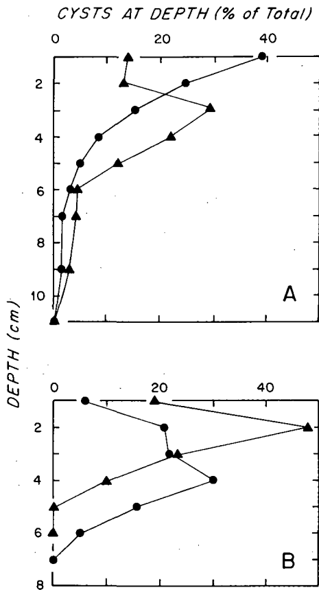
Fig. 4. Vertical distribution of different types of cyst in the same core. A—Cysts of Gonyaulax tamarensis (▲) and Heterocapsa triquetra (●) in Perch Pond. B—Cysts of Gyrodinium uncatenum (▲) and Gyrodinium sp. (tentative identification) (●) in Potomac River.
