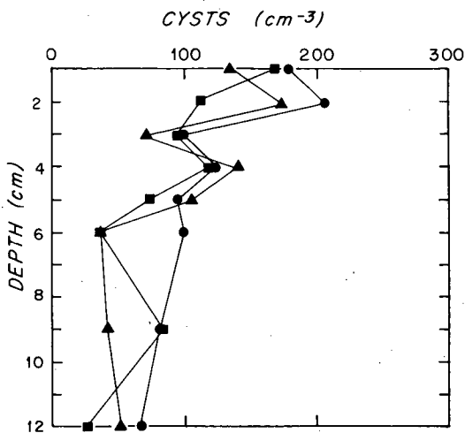
Fig. 3. Vertical profiles of cysts of Gonyaulax scrippsae at 20-m depth in Buzzards Bay: ●—gravity core; ▲—box core; ■—5-cm-diameter subcore from box-core sample. Each point represents a 1-cm interval above specified depth.
