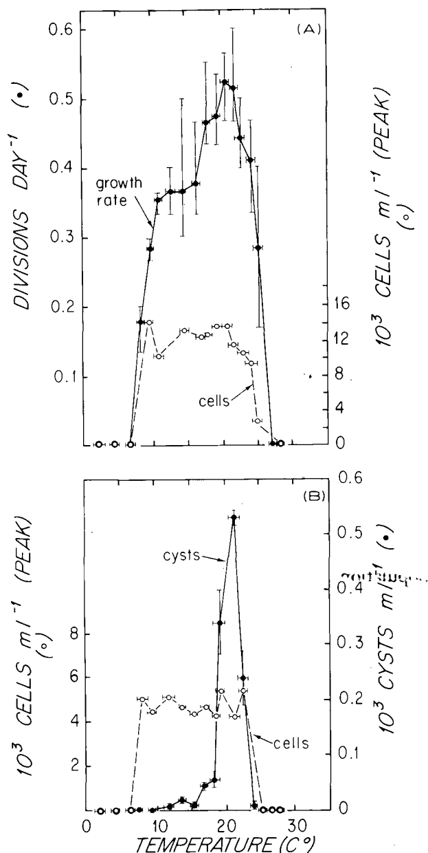
FIG. 2A, B. The effect of temperature on G. tamarensis growth rate, peak motile cell concentration, and cyst production in batch cultures. A. Growth rate (●) and peak cell concentration (○) versus temperature in nutrient-replete f/2-Si medium; B. Cyst yield (●) and peak motile cell concentration (○) versus temperature in ammonium-encystment medium. Vertical error bars show the range of triplicate counts; horizontal error bars indicate the range of temperature fluctuations.
