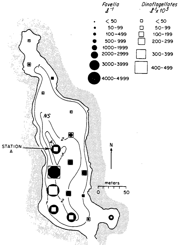
Fig. 1. Horizontal distribution of Favella and dinoflagellates, Perch Pond, May 19, 1982. Depth contours are in meters.
