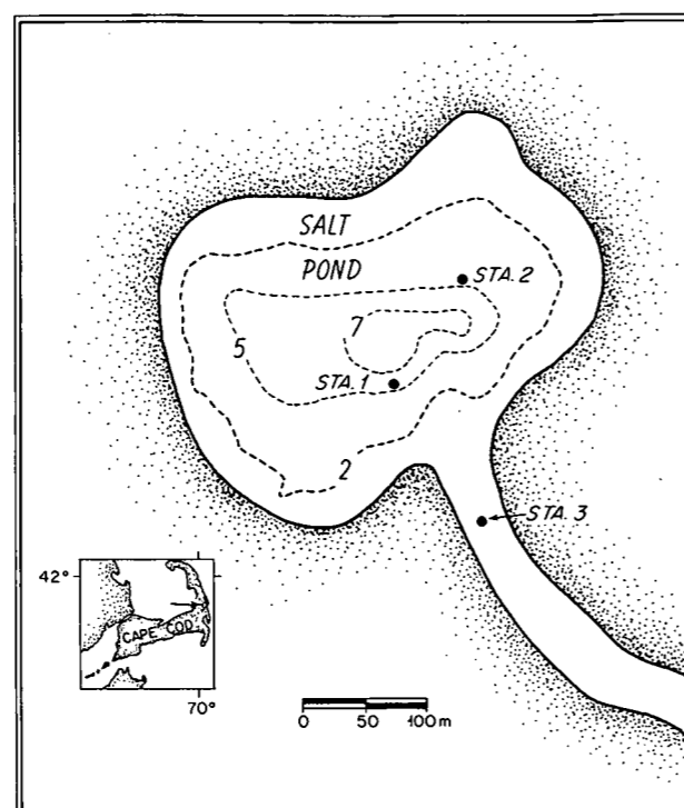
Fig. 1. Map of Salt Pond, Eastham, Massachusetts (USA) with sampling stations. Contours are in m at slack low tide
