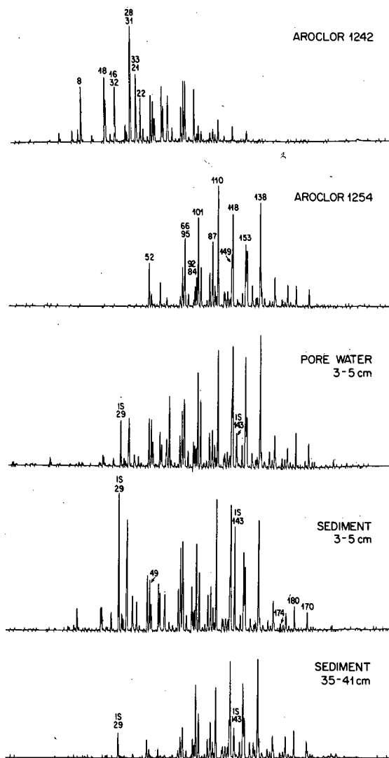
FIG. 2. Capillary gas chromatograms of PCB Aroclor standards, pore water and sediment samples from 3-5 cm depth, and the 35-41 cm sediment sample. Retention times increase along the x-axis. Chlorobiphenyl numbers indicate identification of peaks used in total Aroclor calculations and other chlorobiphenyls reported here (see Table 2).
