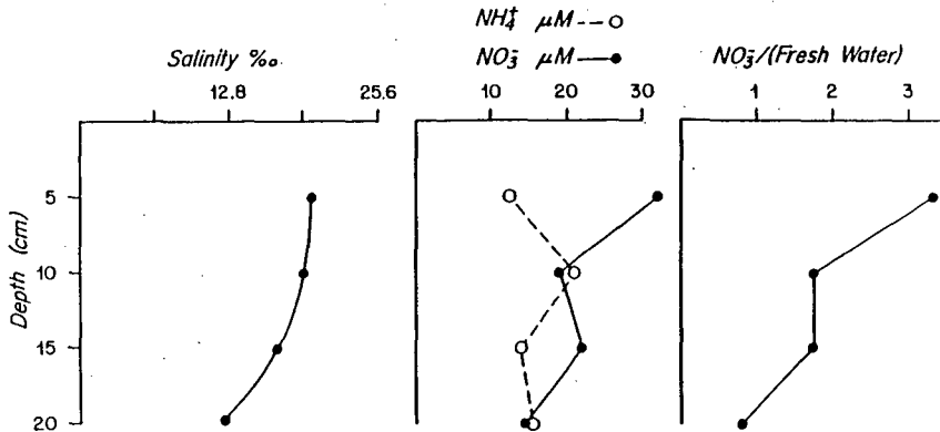
Fig. 6. Profiles of salinity, ammonia, and nitrate in sediment porewater. The ratio of nitrate/fresh-water is defined as [nitrate/(30-salinity)].
