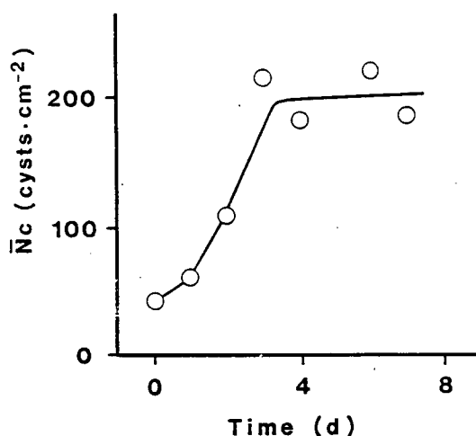
Fig. 2. Time course of Chattonella antiqua encystment. \bar{N}_c , Average cyst yield on coverslips ( n=8 or 12). At t=0 , cultures were placed in continuous darkness. SD of N_c was ca. 50% of \bar{N}_c .
