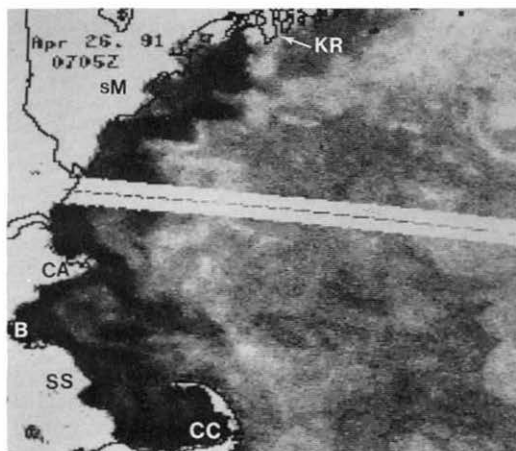
FIG. 3. NOAA Coastwatch SST image from April 26, 1991 at 0305 hrs local time during an early spring runoff event. The warmer (darker) plume extends along the coast. Shellfish toxicity was detected only in southern Maine (sM) at this time. Low concentrations of A. tamarensis were detected within the plume further to the south, but well offshore in Massachusetts Bay just north of Cape Cod (CC).
