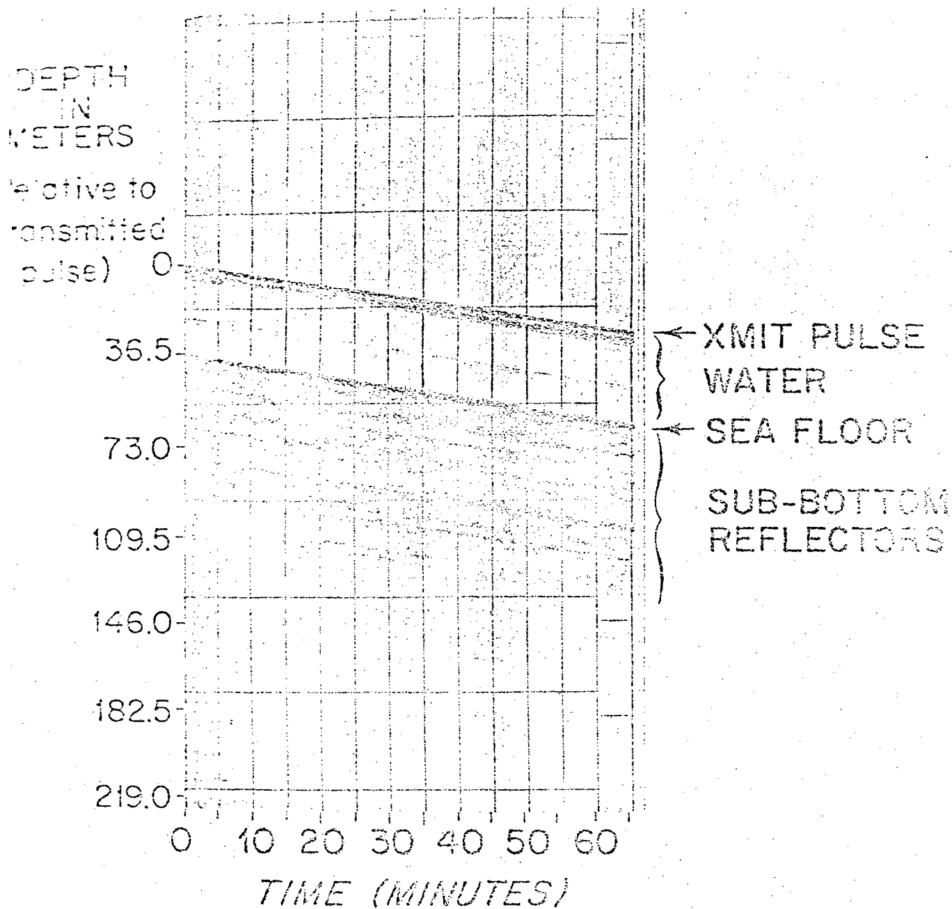
Fig. I DEEP ECHO SOUNDER PGR M RECORD MADE NEAR BERMUDA IN 1965
