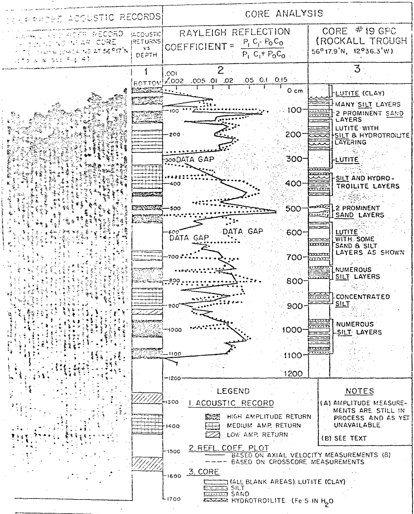
Fig. II ACOUSTIC RECORDS VS CORE ANALYSIS
