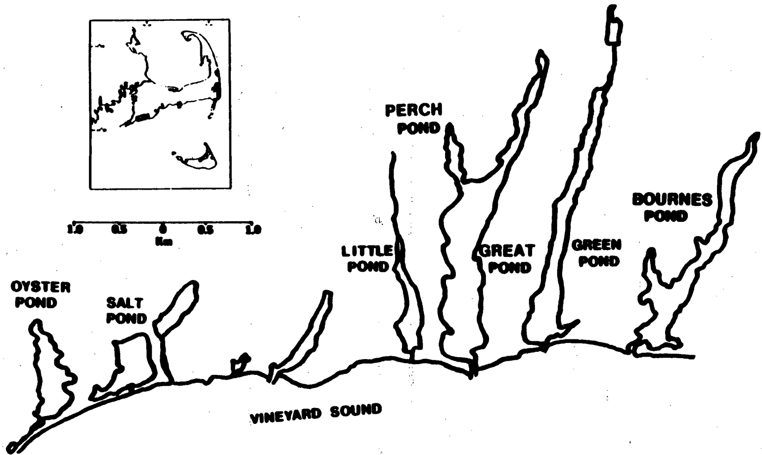
Figure 1. Relative locations of the coastal salt ponds in Falmouth, Massachusetts.
