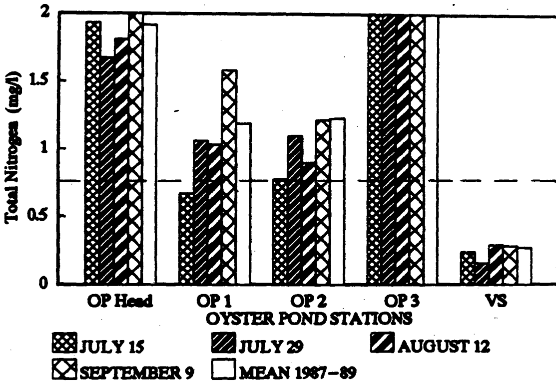
Figure 8a, b & c. Water column weighted averages of total nitrogen in each of the four samplings in 1990 versus the average of summer samplings from 1987-1989. Note the initially low values on July 15 with increasing levels in later samples. Arrows represent periods when low levels of dissolved oxygen (less than 5 mg/l, generally less than 3) were measured. VS represents Vineyard Sound levels; dashed line represents Nutrient Overlay Bylaw threshold limits of 0.32 mg/l ("High Quality Areas"), 0.50 mg/l ("Stabilization Areas") and 0.75 mg/l ("Intensive Water Activity Areas").
