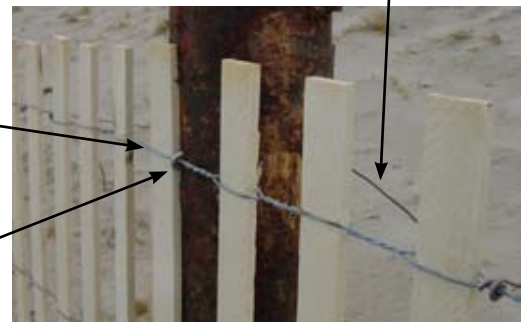
Figure 14. A wire is wrapped around the back of the post and is attached to the sand fence wire approximately 8" to either side. This adds support to the fence under strong wind conditions. A loose attachment allows the fence wire to slide and move to prevent breakage as wind shakes the fence.
